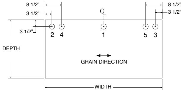
Applies to: Rectangulars, Extended Rectangulars, Cockpit Returns, 120° Returns
