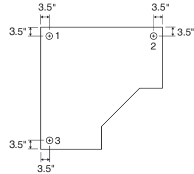
Applies to: All Corners (Rectilinear, Curvilinear, Depth Transitions, Cockpit Corners, 120° Corners, 135° Corners, Corner Keyboards)
