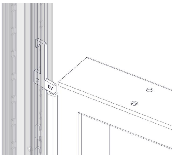
3c: Make sure the locking clip is properly seated as shown and the O-leg is secured to hanger frame.
