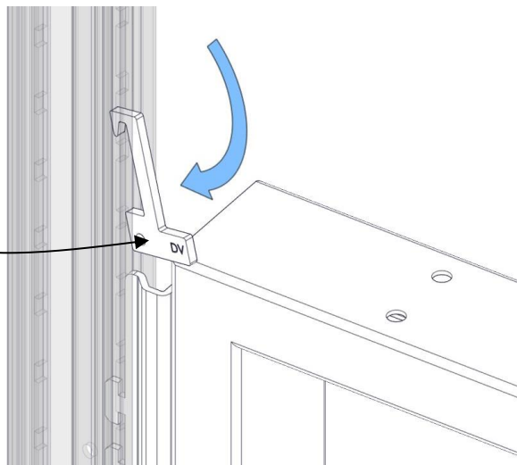
3b: Hook the Locking Clip into the hanger frame slot and rotate down.
